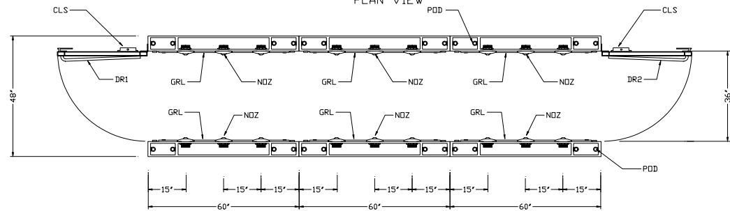
PLAN VIEW
